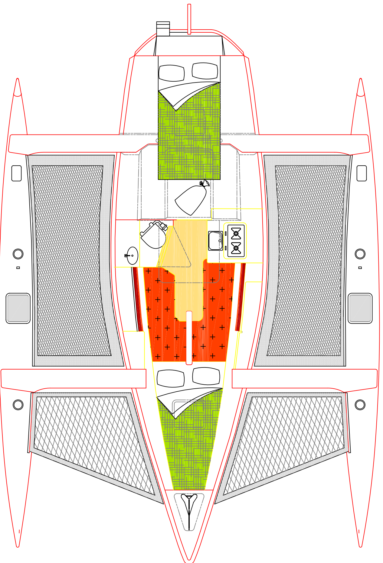
— ACCOMMODATION PLAN — CORSAIR 28CR CENTRE COCKPIT
