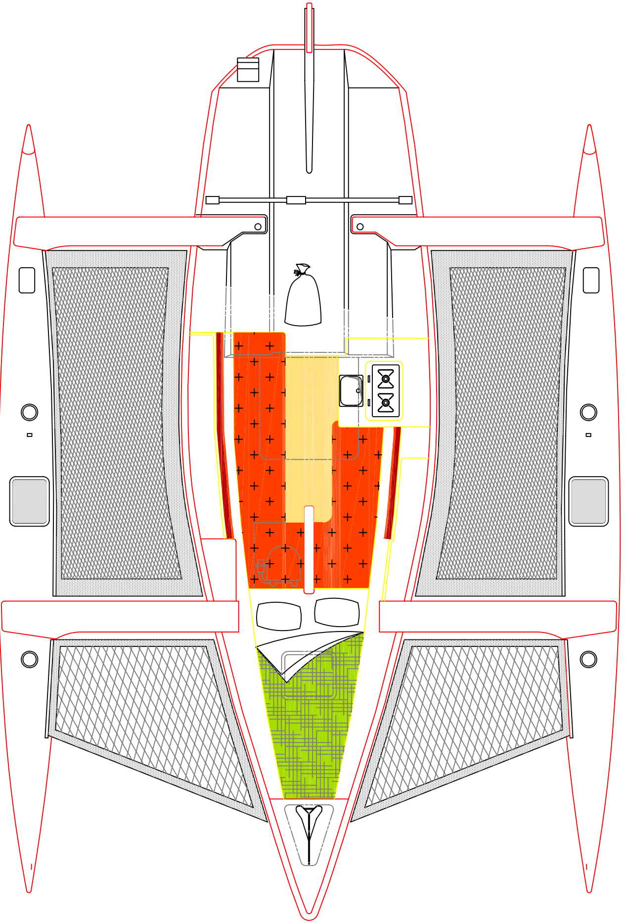
— ACCOMMODATION PLAN — CORSAIR 28RS AFT COCKPIT
